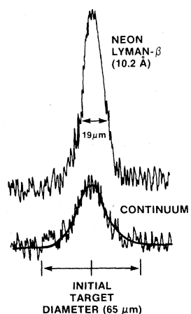
FIG. 5. Spatial profile of the Lyman- \beta line of neon (10.24 Å), and the nearby continuum. The bar indicates the compressed neon diameter as inferred from spectral profiles analysis.
