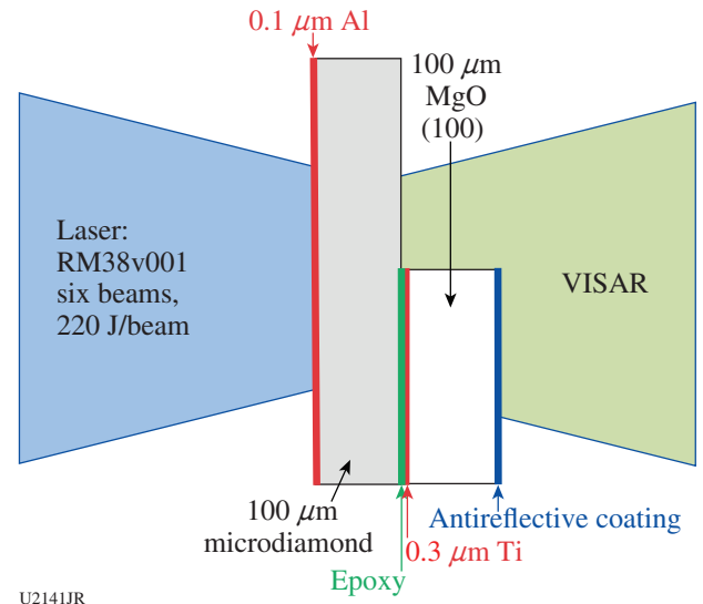
Figure 148.94 Target design for the MaxOxWindow-16A experiment.
