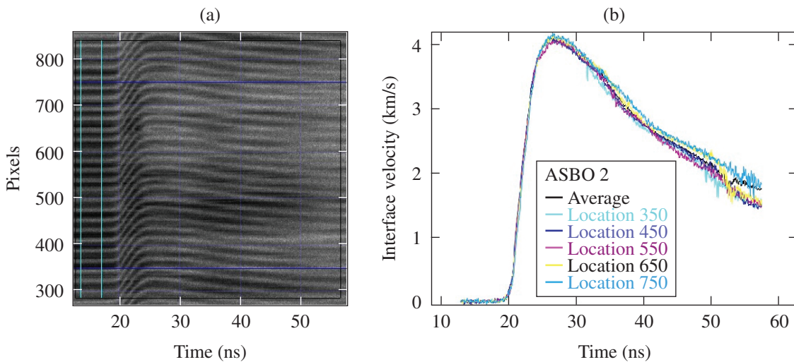
Figure 148.112 (a) The ASBO (VISAR) data from shot 24063 and (b) a series of lineouts taken across the image showing excellent planarity.
