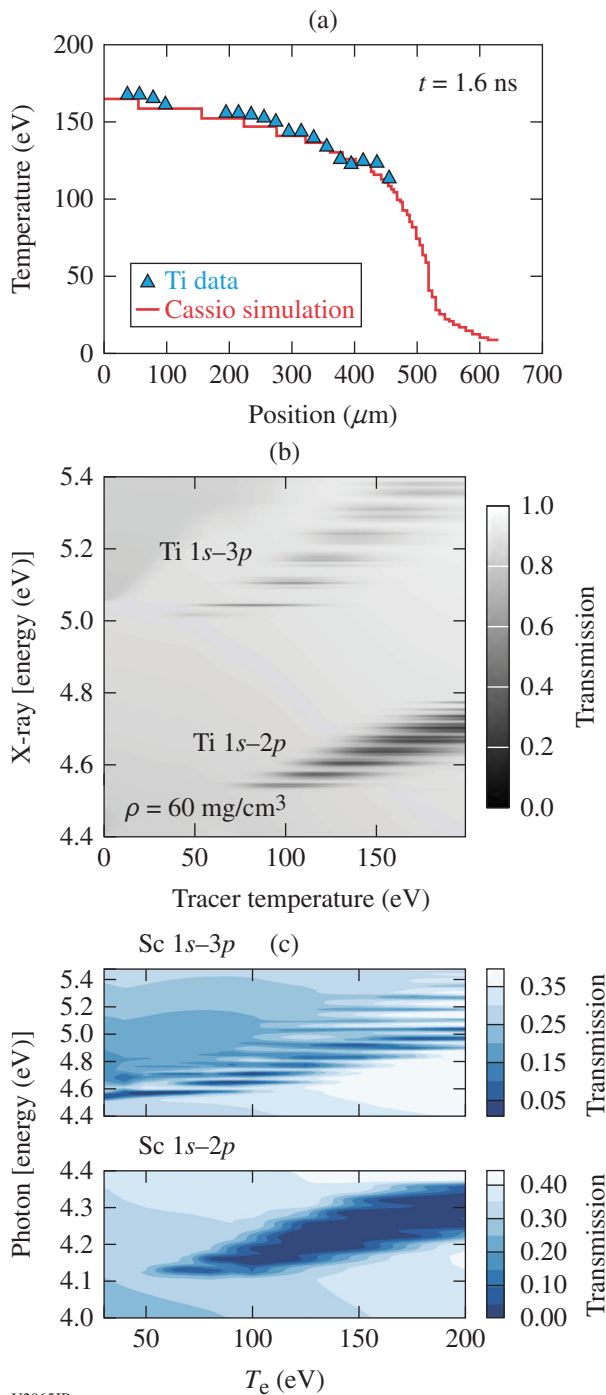
Figure 148.123 (a) The shape of the radiation front in simulation is compared to results from COAX experiments featuring Ti-doped aerogels. Simulated K-shell absorption spectra from PrismSPECT for (b) Ti and (c) Sc illustrate the change in temperature and photon energy distribution of lines for the same transitions in two different elements. These figures were presented at the 2016 High-Temperature Plasma Diagnostics Conference.
