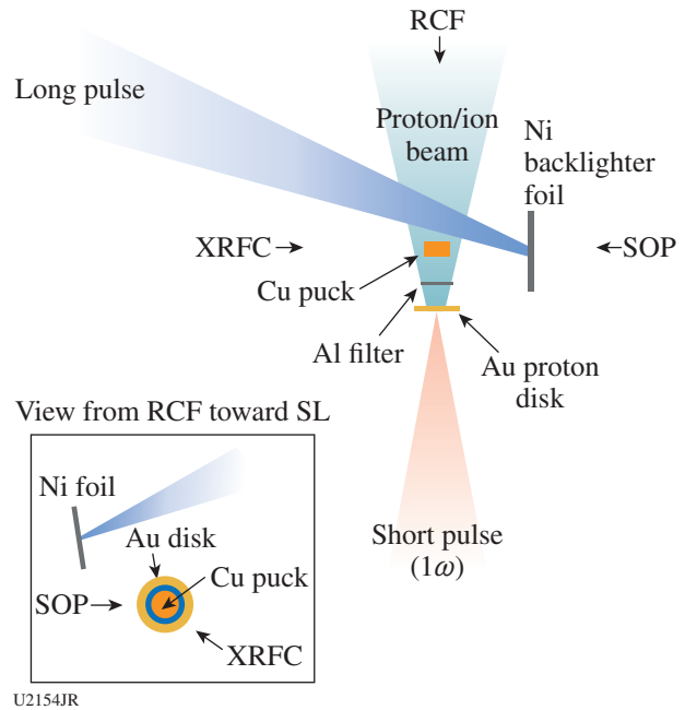
Figure 148.106 Experimental layout for proton-heating shots with combined x-ray radiography, SOP, and radiochromic film (RCF). For simplicity, only one backlighter beam (of the three used) is shown. SL: sidelighter.
