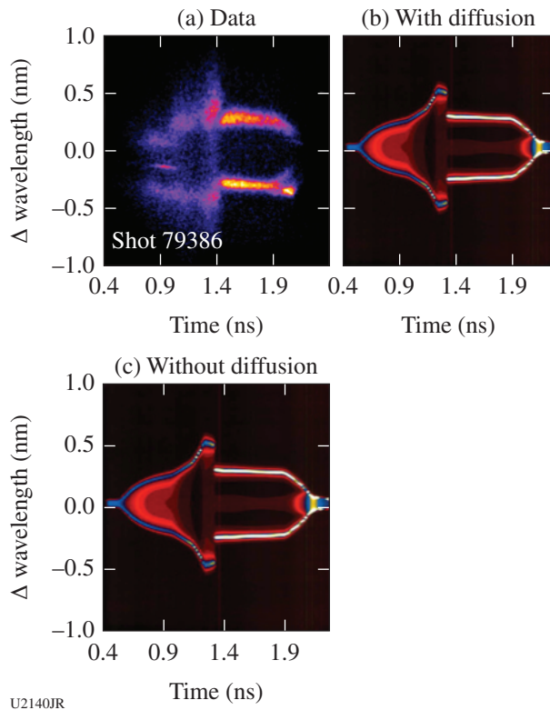
Figure 148.93 The (a) measured Thomson-scattering signal is compared to post-shot simulations (b) using or (c) not using a diffusion model to investigate the interpenetration of Au into the CH plasma.
