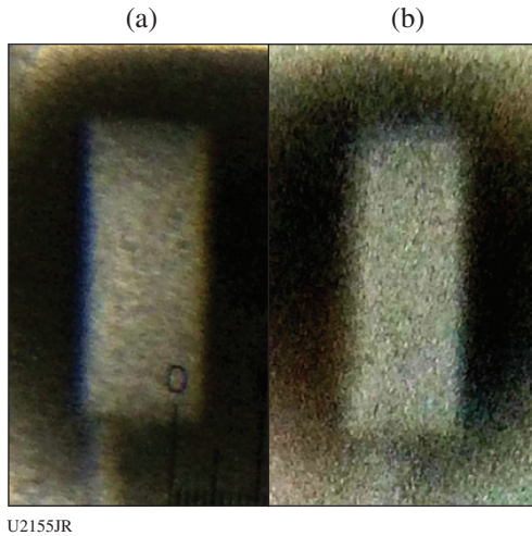
Figure 148.107 Gated x-ray imaging data from (a) an unheated and (b) a heated copper foam puck. For the heated shot, the backlighter was delayed by 20 ns. From this perspective, the protons propagate from left to right through the target. There is clear expansion of the front surface in (b).
