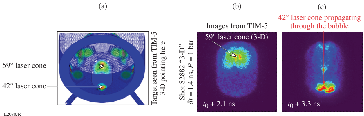
Figure 148.143 Images obtained with the hard x-ray imager in TIM-5 (P8 configuration).
