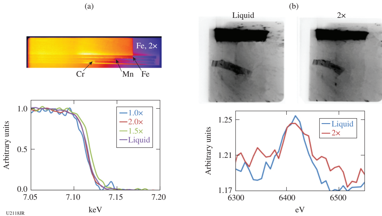
Figure 148.78 (a) A raw image of the measured absorption spectrum for 2× compressed Fe and measured Fe K edge under four different conditions. (b) Top: Measured MSPEC spectra, despeckled to reduce noise. Bottom: Lineouts of the Fe K_{\alpha} feature for liquid and 2× compressed Fe.
