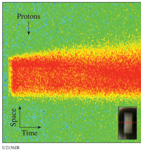
Figure 148.108 SOP data from a proton-heating shot. The insert shows the position and orientation of the SOP slit relative to the target. There is a clear difference between the expansion of the front (proton-facing) and rear surfaces.
