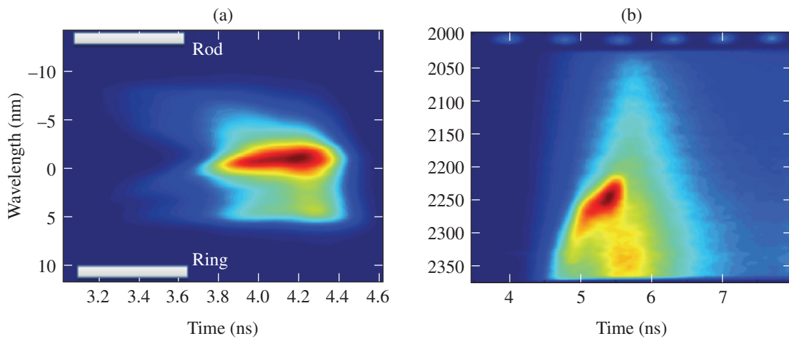
Figure 148.87 (a) Ion-acoustic wave (IAW) and (b) electron plasma wave (EPW) spectra for carbon into carbon.
