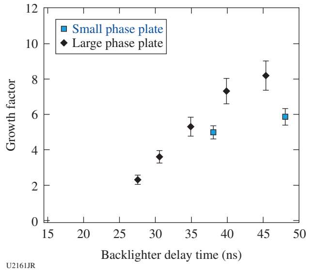
Figure 148.113 Growth factor data for solid copper using small and large phase plates.
