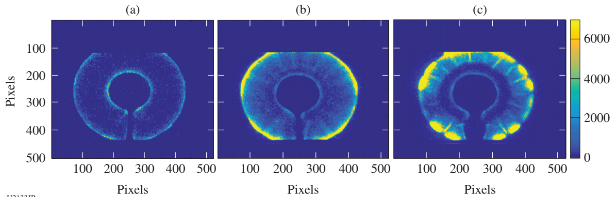
Figure 148.86 X-ray images at 0.9 ns for the three different rings: (a) carbon, (b) aluminum, and (c) gold. The center circle is the high-density carbon ring; the outer circle is the low- to high-Z ring.
