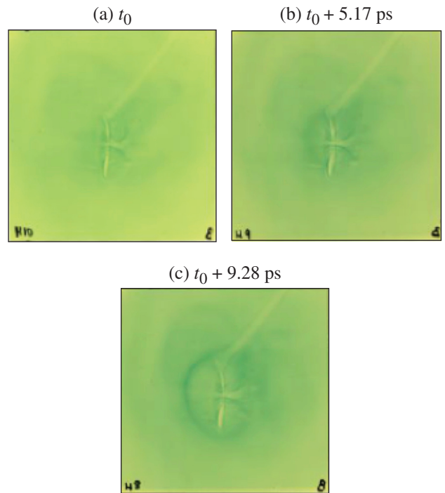
Figure 148.64 Proton images of target normal geometry
