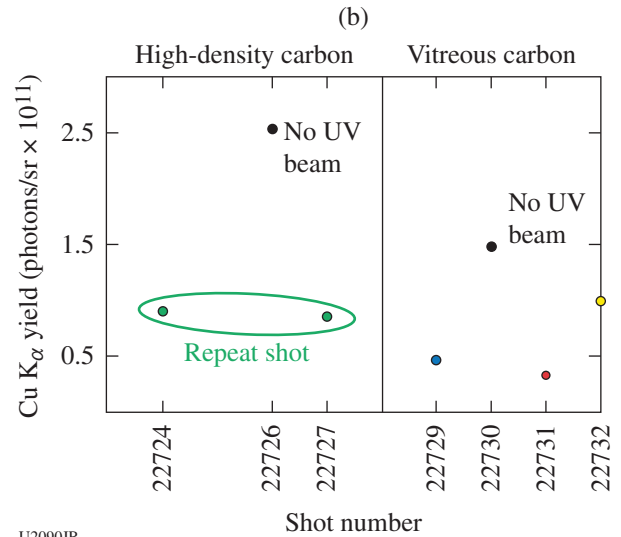
Figure 148.43 (a) SCI spatial profile of fluorescence emission from copper in HDC shots, showing evidence of a focused electron beam with bright localized emission when the target is initially shock heated. (b) Plot of Cu K_{\alpha} photon yield calculated from spectra recorded on the calibrated zinc von Hamos x-ray spectrometer. While the overall signal drops when the targets are initially heated, this is likely caused by the refluxing of electrons over the entire target, as seen in the SCI data. The red, blue, and yellow dots correspond to a shock position 1/5, 2/3, and fully through the carbon target layer, respectively.
